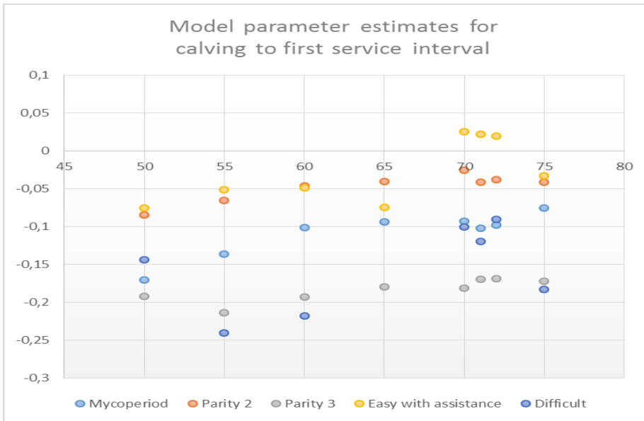
Figure 4 A plot of the parameter estimates (y-axis) with different break points for dichotomized calving to first service intervals.
